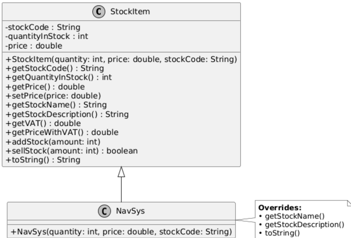
UML Diagram Version 2 – StockItem + NavSys (Part 2.1)
