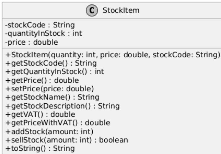
UML Diagram Version 1 – StockItem Class Only (Part 1.1)
